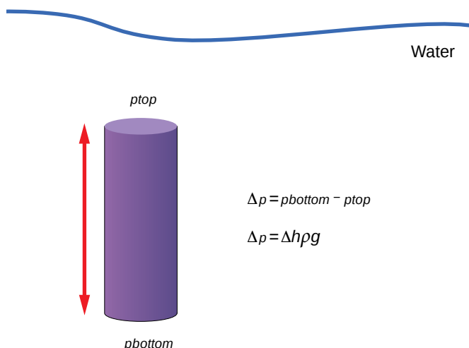
Figure 6.45 The pressure difference = \Delta h\rho g
