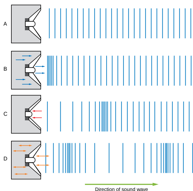
Figure 8.43 How a speaker produces a sound wave
