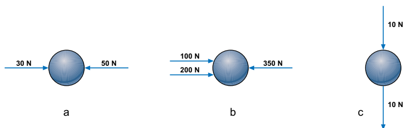
Figure 1.24 Examples for Question 1
