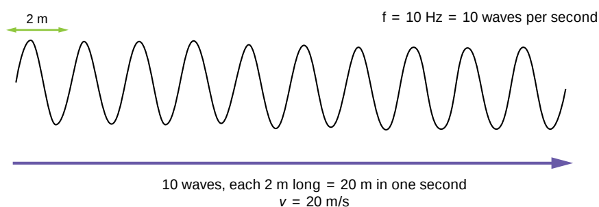
Figure 8.30 Showing how v = f\lambda
