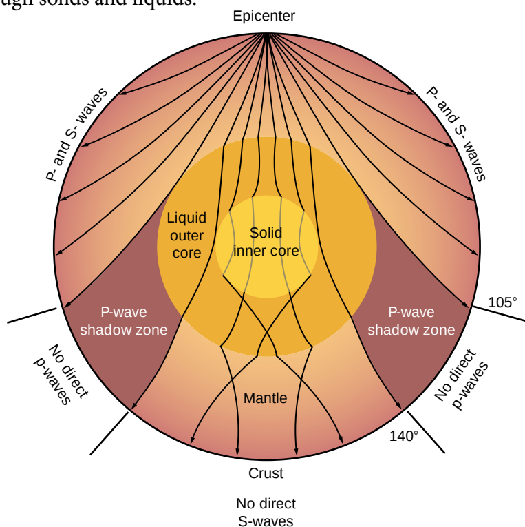
Figure 8.27 Using seismic waves to determine the structure of the Earth
