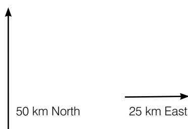
Figure 1.2 Two different displacement vectors, represented by arrows.
