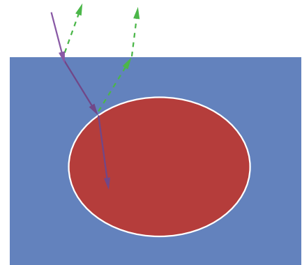
Figure 8.61 The reflection and refraction of sound through different materials
