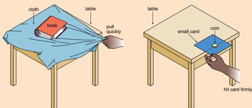
Figure 3.12 Demonstrating inertia
