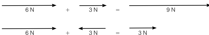
Figure 1.4 Parallel vector addition (along a line). The resultant is 9 N if they are in the same direction but 3 N if the forces are in opposite directions.
