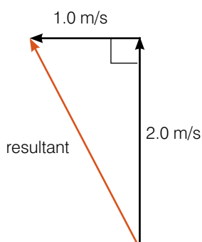
Figure 1.10 The swimmer's velocity vectors shown as a right-angled triangle.
