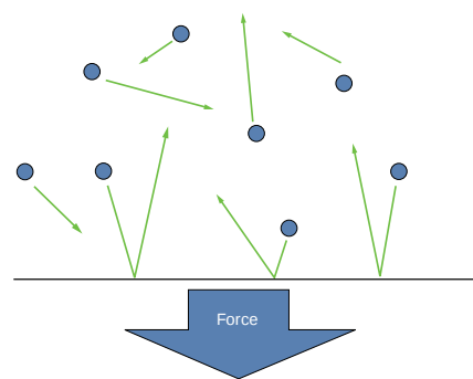
Figure 6.5 Air particles crashing into a surface apply a force to that surface.
