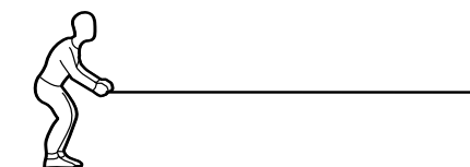
Figure 8.7 A simple wave pulse
