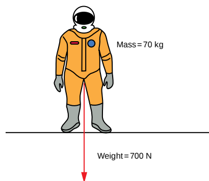
Figure 3.44 Weight and mass
