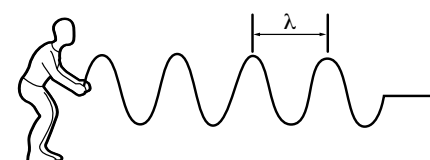
Figure 8.8 A simple continuous wave
