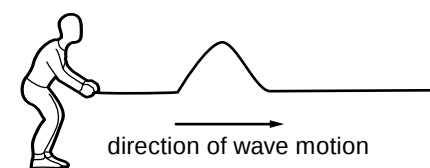
Figure 8.7 A simple wave pulse
