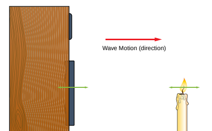
Figure 8.42 Demonstrating sound waves are longitudinal
