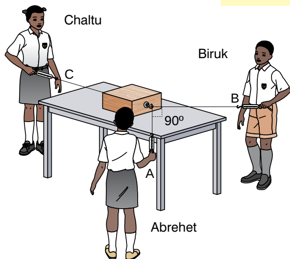
Figure 1.31 Investigating vectors
