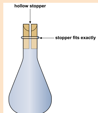
Figure 6.25 A density bottle
