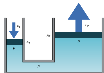
Figure 6.34 Pascal's principle
