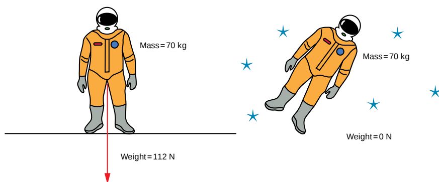
Figure 3.45 Astronaut on the Moon and in deep space
