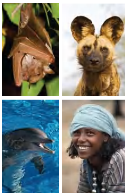
Figure 8.44 Different animals have different audible ranges.
