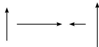
Figure 1.23 Four components from the two vectors in Figure 1.22
