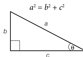
Figure 1.9 A right-angled triangle
