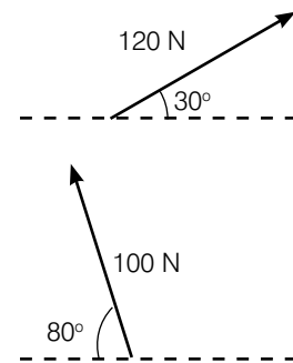
Figure 1.22 Two vectors at different angles
