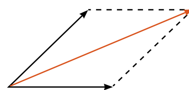
Figure 1.15 Parallelogram method for non-perpendicular vectors
